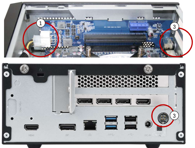
XH510G2 with two power adapters connected Graphics card: MSI GeForce RTX 3060 AERO ITX 12G OC
