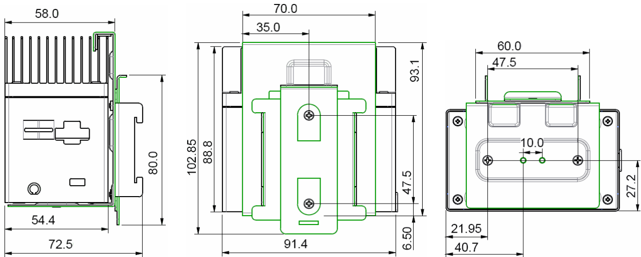
VESA Mount
