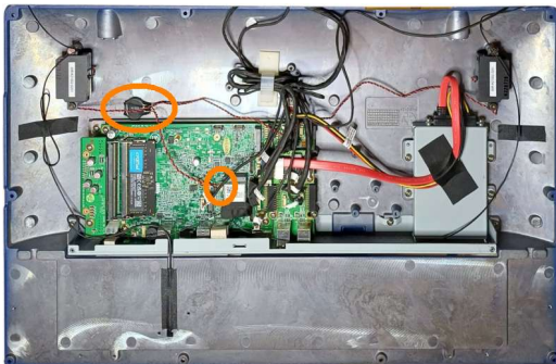
Photo: Position of the button cell battery and the connector on the mainboard with the computer housing open.
