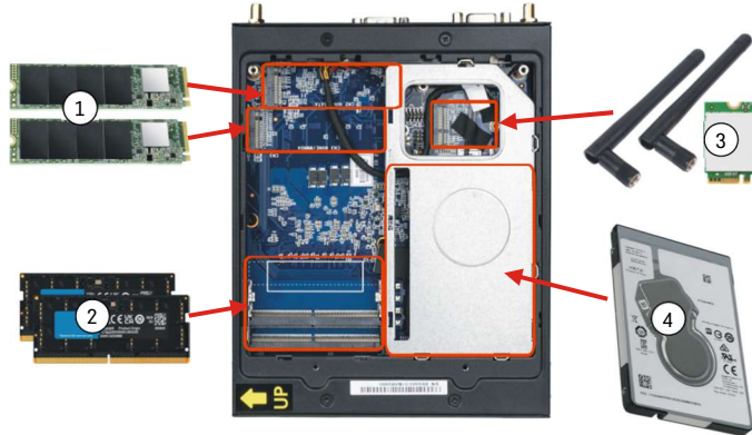
Shuttle XPC slim Barebone DS50U5 with opened chassis
